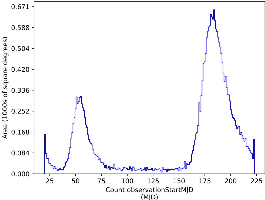
too_elab_r16_d3_giz_v3.4_10yrs r: Count observationStartMJD
