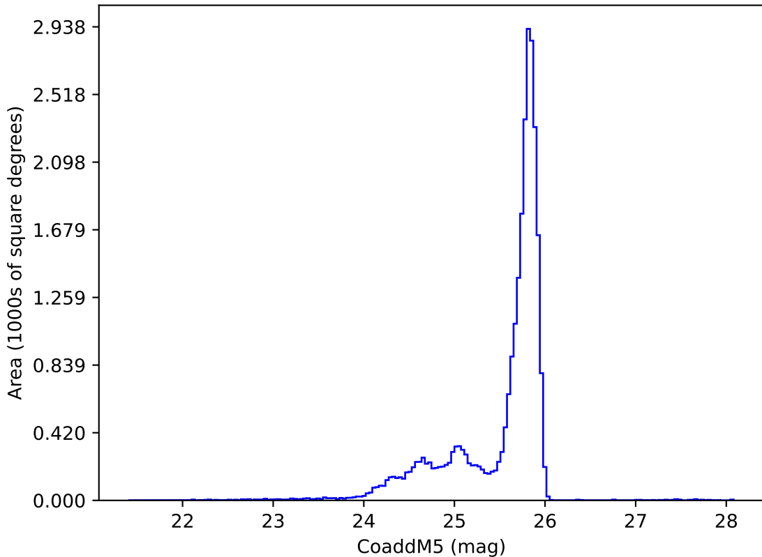
too_elab_r16_d3_giz_v3.4_10yrs z: CoaddM5
