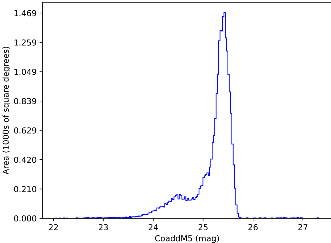
too_elab_r16_d3_giz_v3.4_10yrs u: CoaddM5
