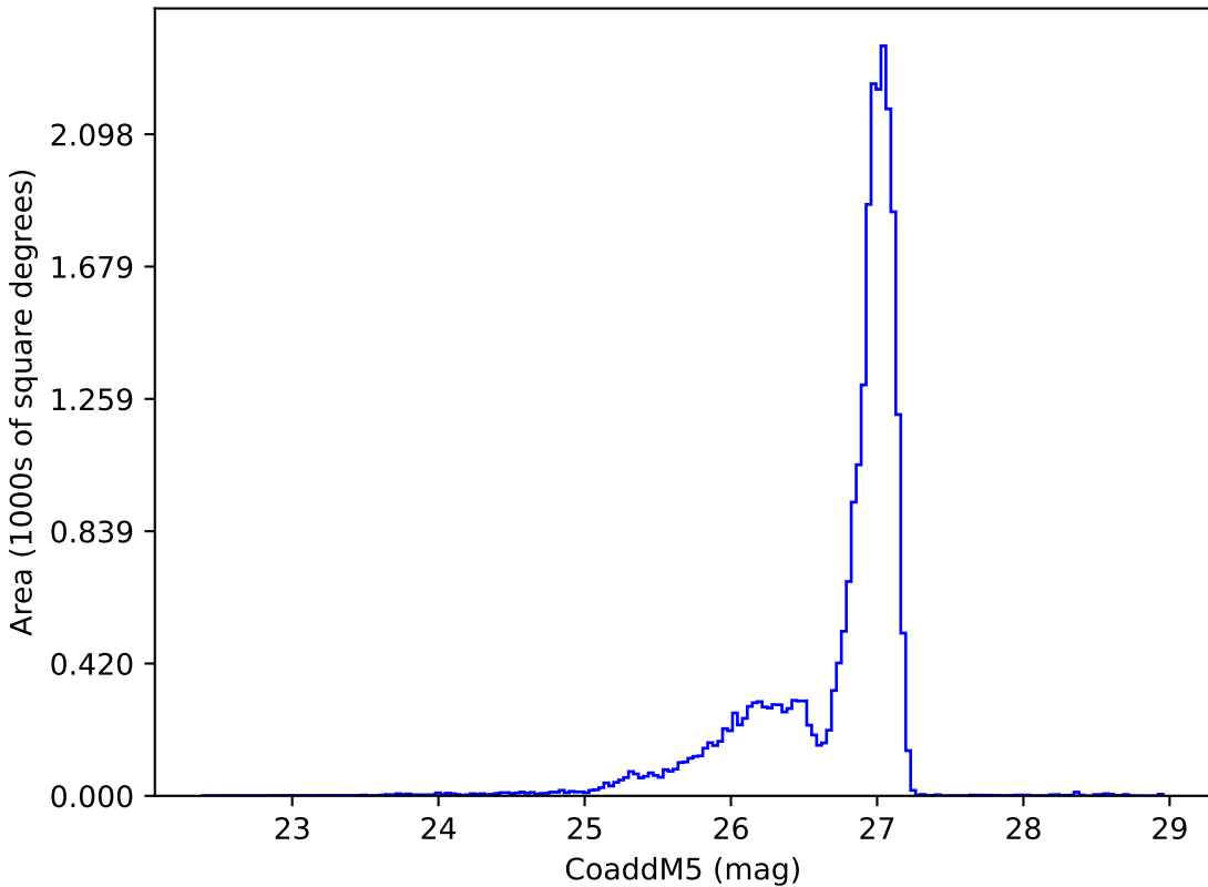
too_elab_r16_d3_giz_v3.4_10yrs r: CoaddM5
