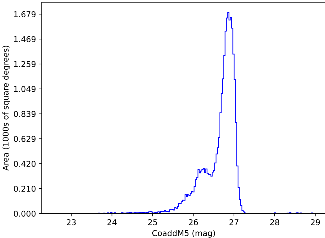
too_elab_r16_d3_giz_v3.4_10yrs g: CoaddM5
