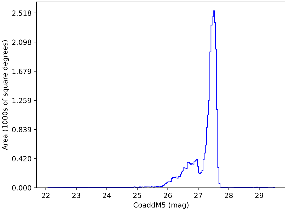
too_elab_r16_d3_giz_v3.4_10yrs : CoaddM5
