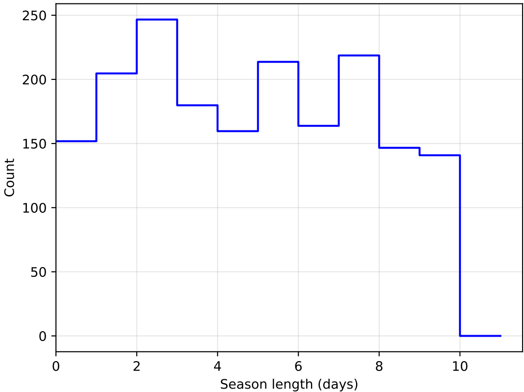
too_elab_r16_d3_giz_v3.4_10yrs DD:WFD all bands: SeasonLength
