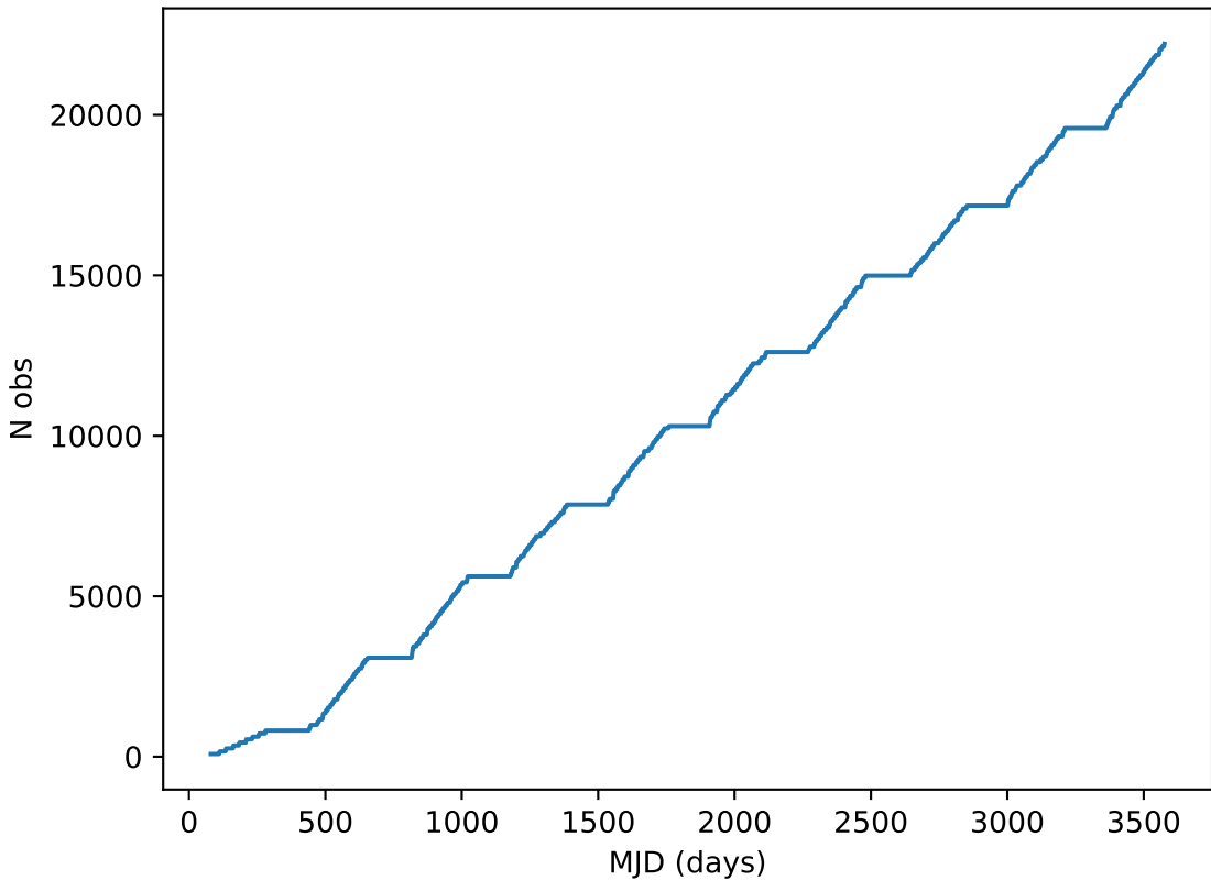
too_elab_r16_d3_giz_v3.4_10yrs all bands: DD:XMM_LSS Cumulative NVisits
