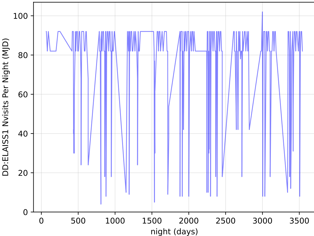
too_elab_r16_d3_giz_v3.4_10yrs all bands: DD:ELAISS1 Nvisits Per Night
