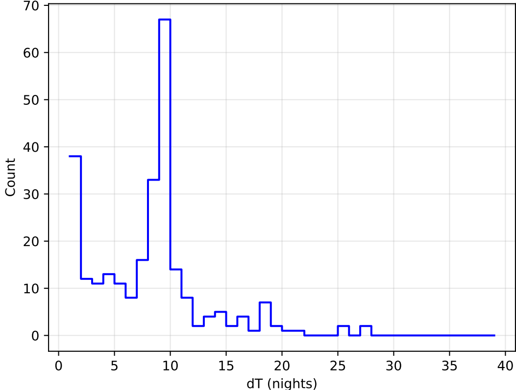
too_elab_r16_d3_giz_v3.4_10yrs all bands: DD:ELAISS1 Delta Nights Histogram
