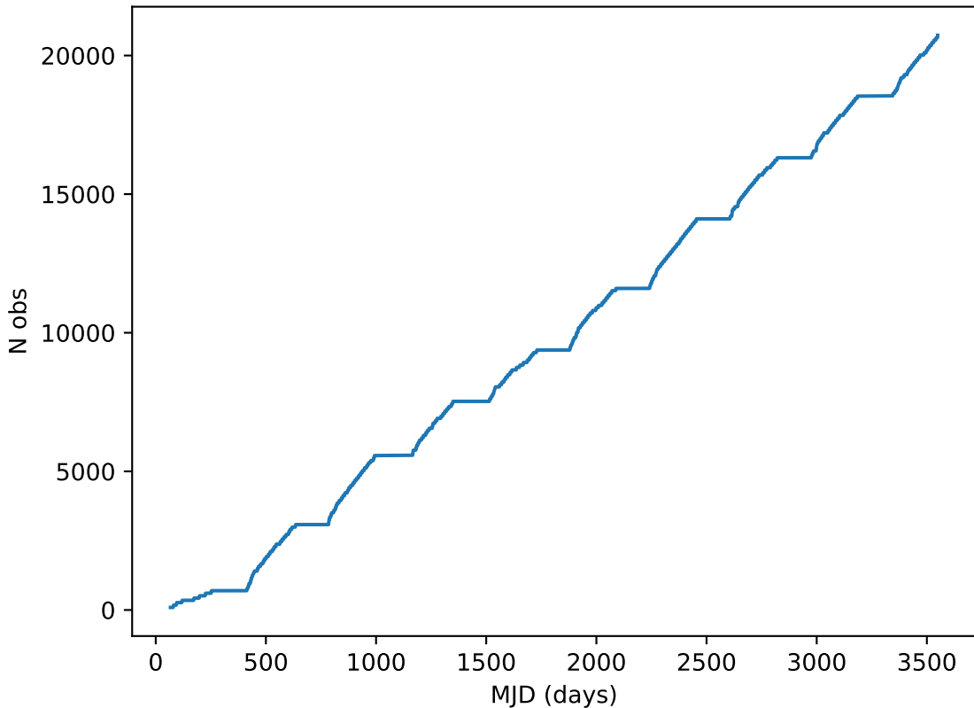
too_elab_r16_d3_giz_v3.4_10yrs all bands: DD:ELAISS1 Cumulative NVisits
