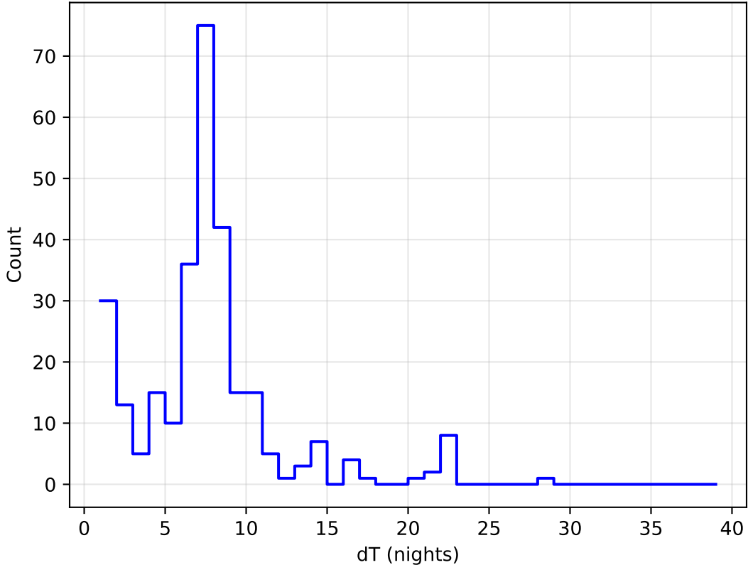
too_elab_r16_d3_giz_v3.4_10yrs all bands: DD:EDFS Delta Nights Histogram
