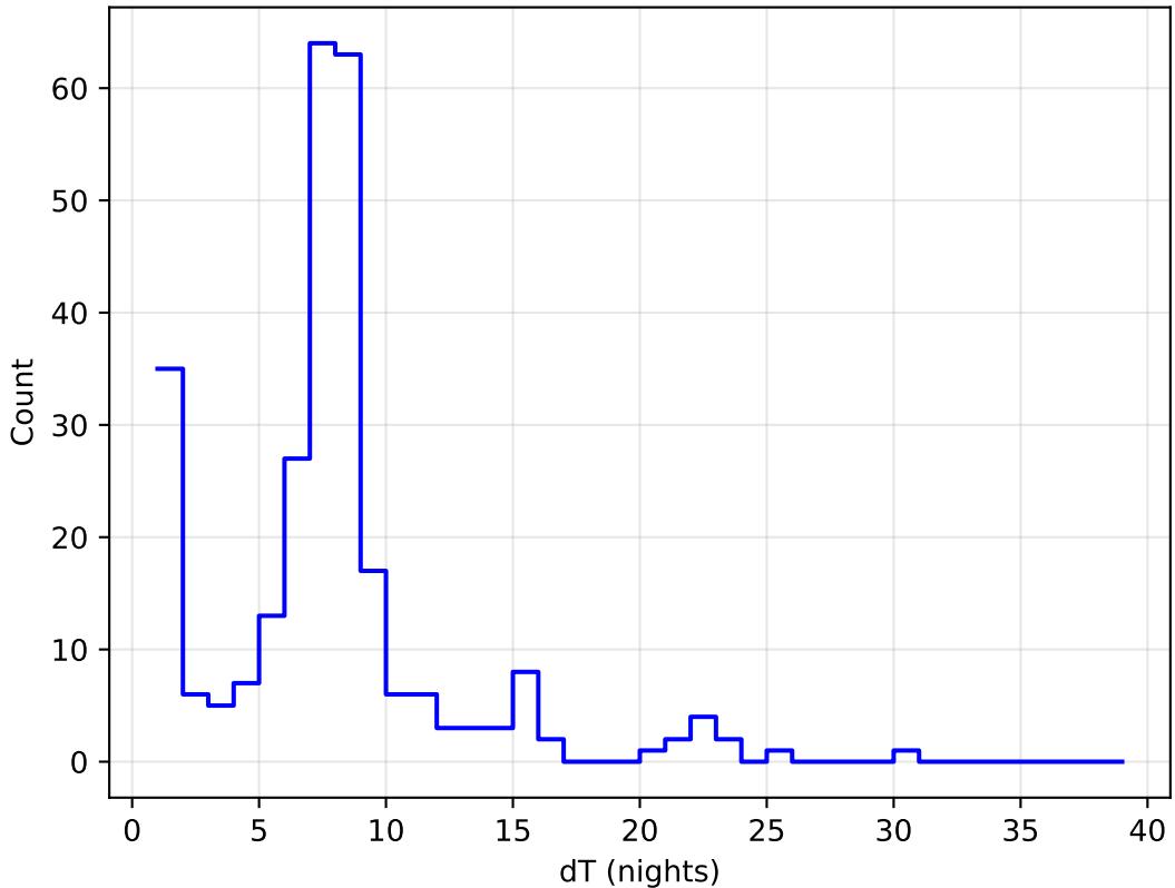
too_elab_r16_d3_giz_v3.4_10yrs all bands: DD:ECDFS Delta Nights Histogram
