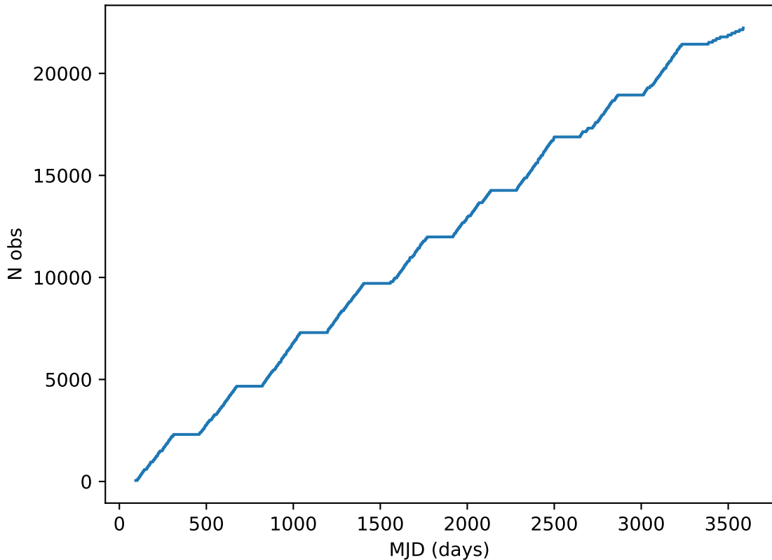
too_elab_r16_d3_giz_v3.4_10yrs all bands: DD:ECDFS Cumulative NVisits
