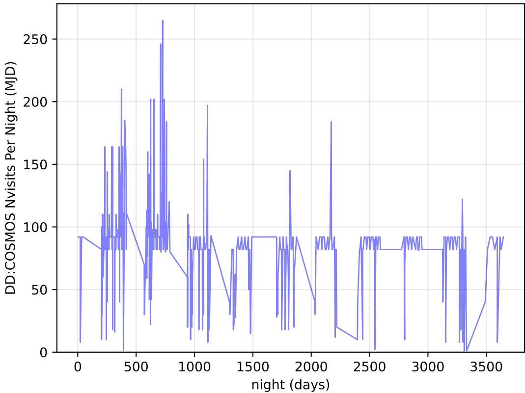
too_elab_r16_d3_giz_v3.4_10yrs all bands: DD: COSMOS Nvisits Per Night
