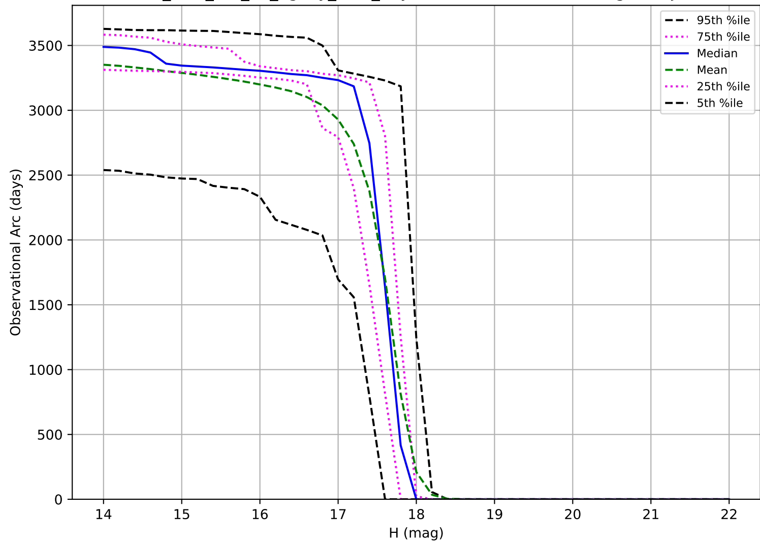
too_elab_r16_d2_ugrizy_v3.4_10yrs: Observational Arc Length Trojan
