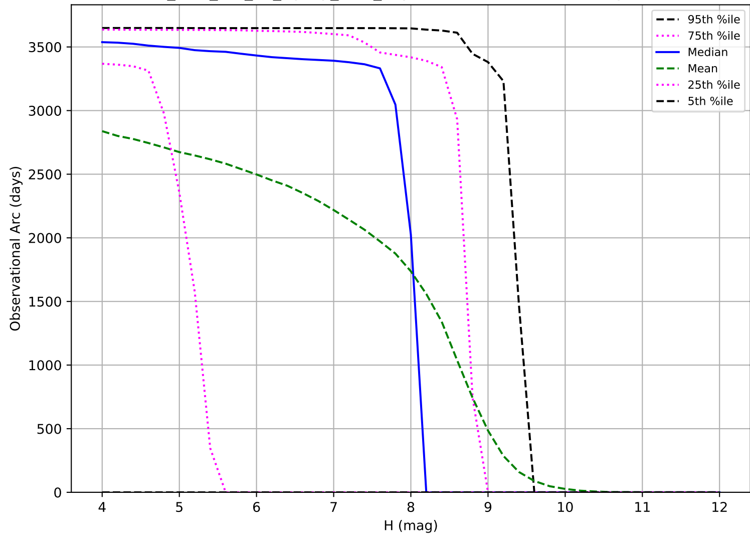
too_elab_r16_d2_ugrizy_v3.4_10yrs: Observational Arc Length TNO
