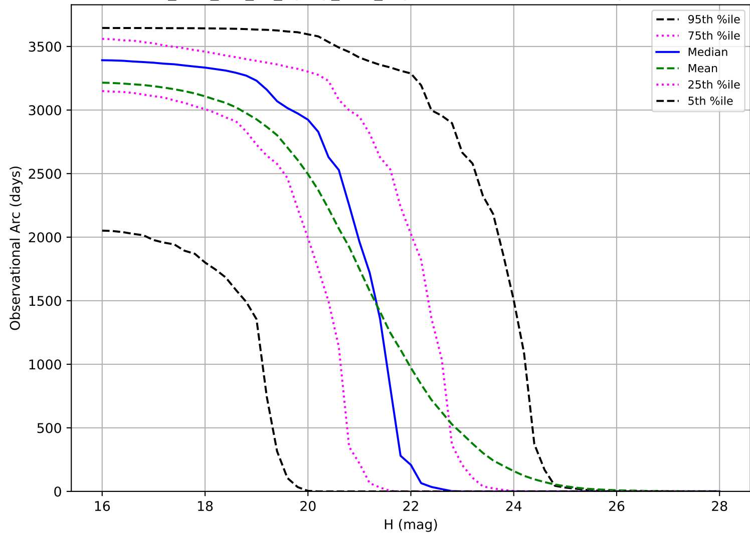
too_elab_r16_d2_ugrizy_v3.4_10yrs: Observational Arc Length PHA
