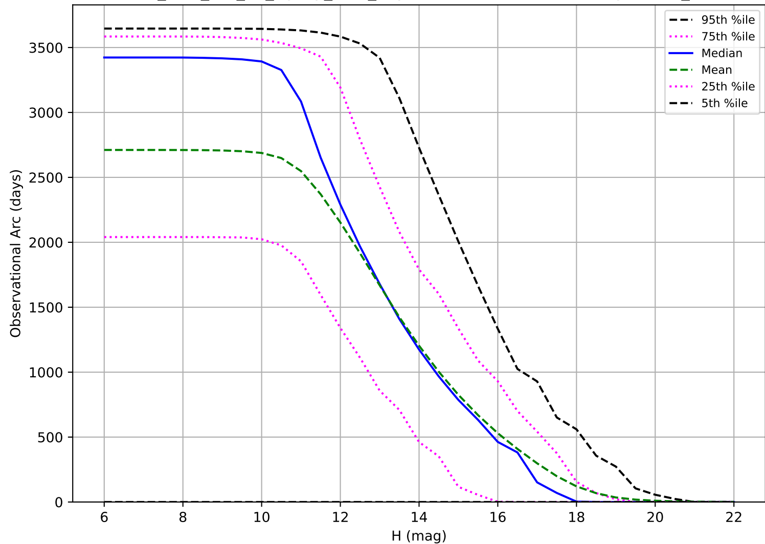
too_elab_r16_d2_ugrizy_v3.4_10yrs: Observational Arc Length OCC_r5
