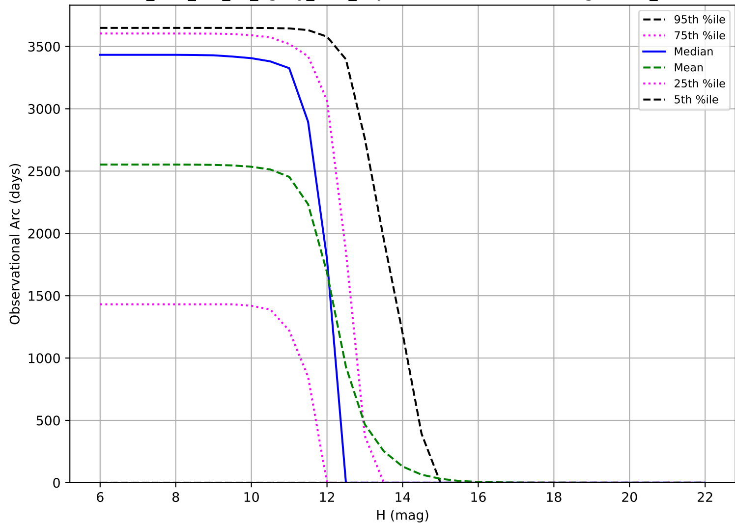
too_elab_r16_d2_ugrizy_v3.4_10yrs: Observational Arc Length OCC_r20
