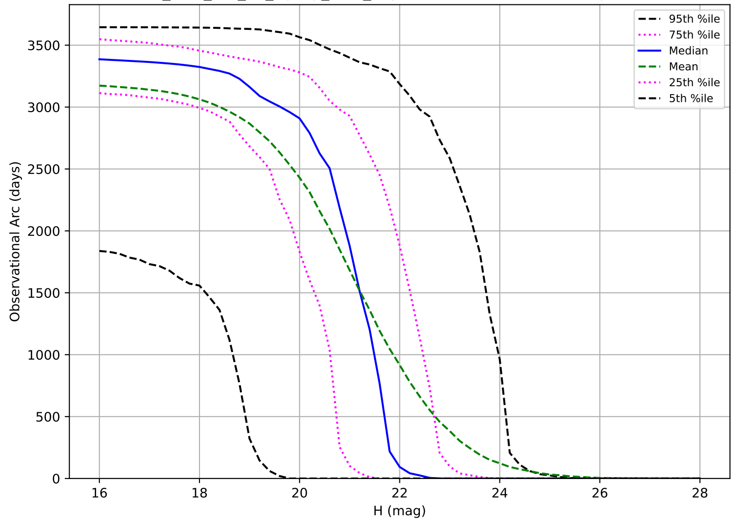
too_elab_r16_d2_ugrizy_v3.4_10yrs: Observational Arc Length NEO
