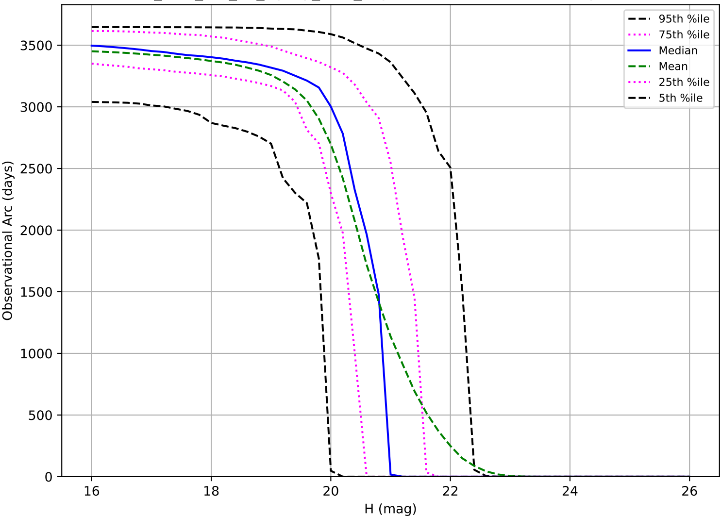
too_elab_r16_d2_ugrizy_v3.4_10yrs: Observational Arc Length MBA
