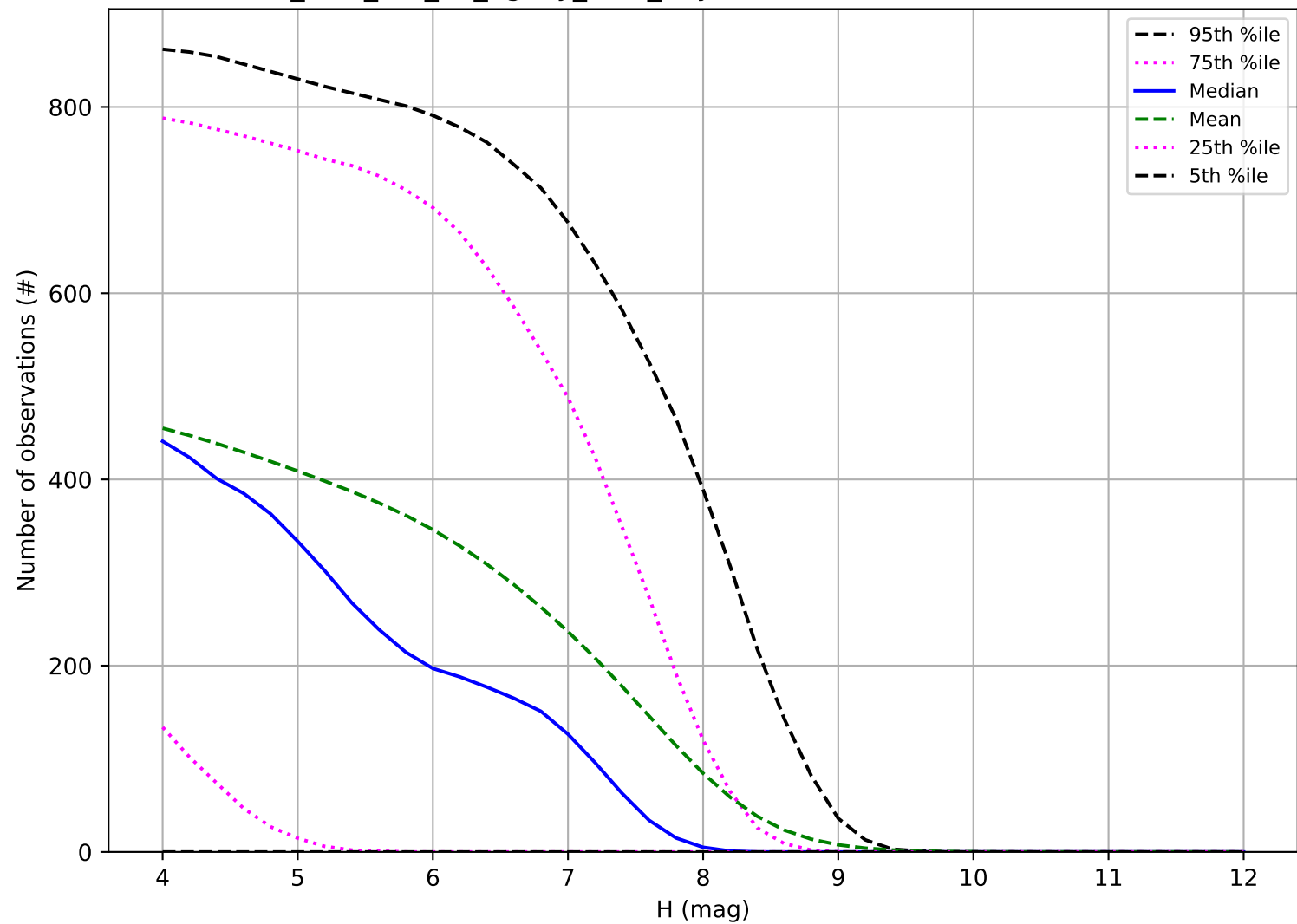
too_elab_r16_d2_ugrizy_v3.4_10yrs: Number of observations TNO
