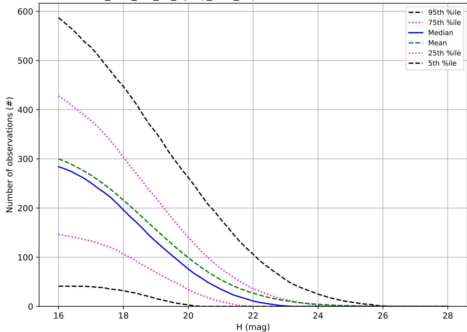
too_elab_r16_d2_ugrizy_v3.4_10yrs: Number of observations PHA
