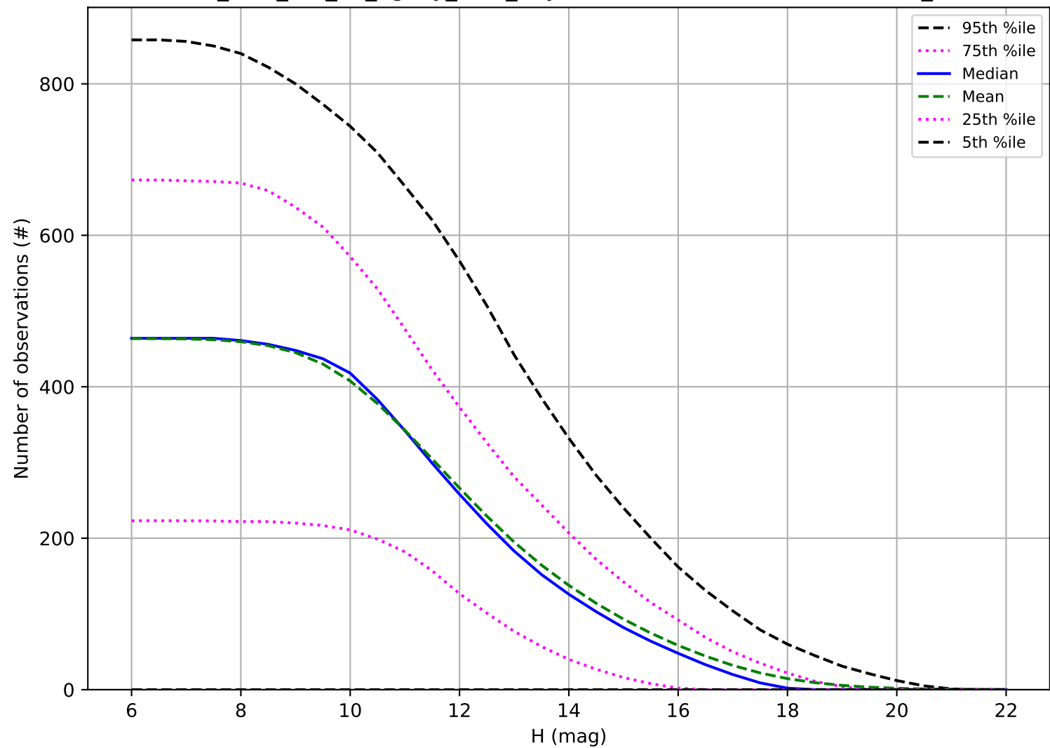
too_elab_r16_d2_ugrizy_v3.4_10yrs: Number of observations OCC_r5
