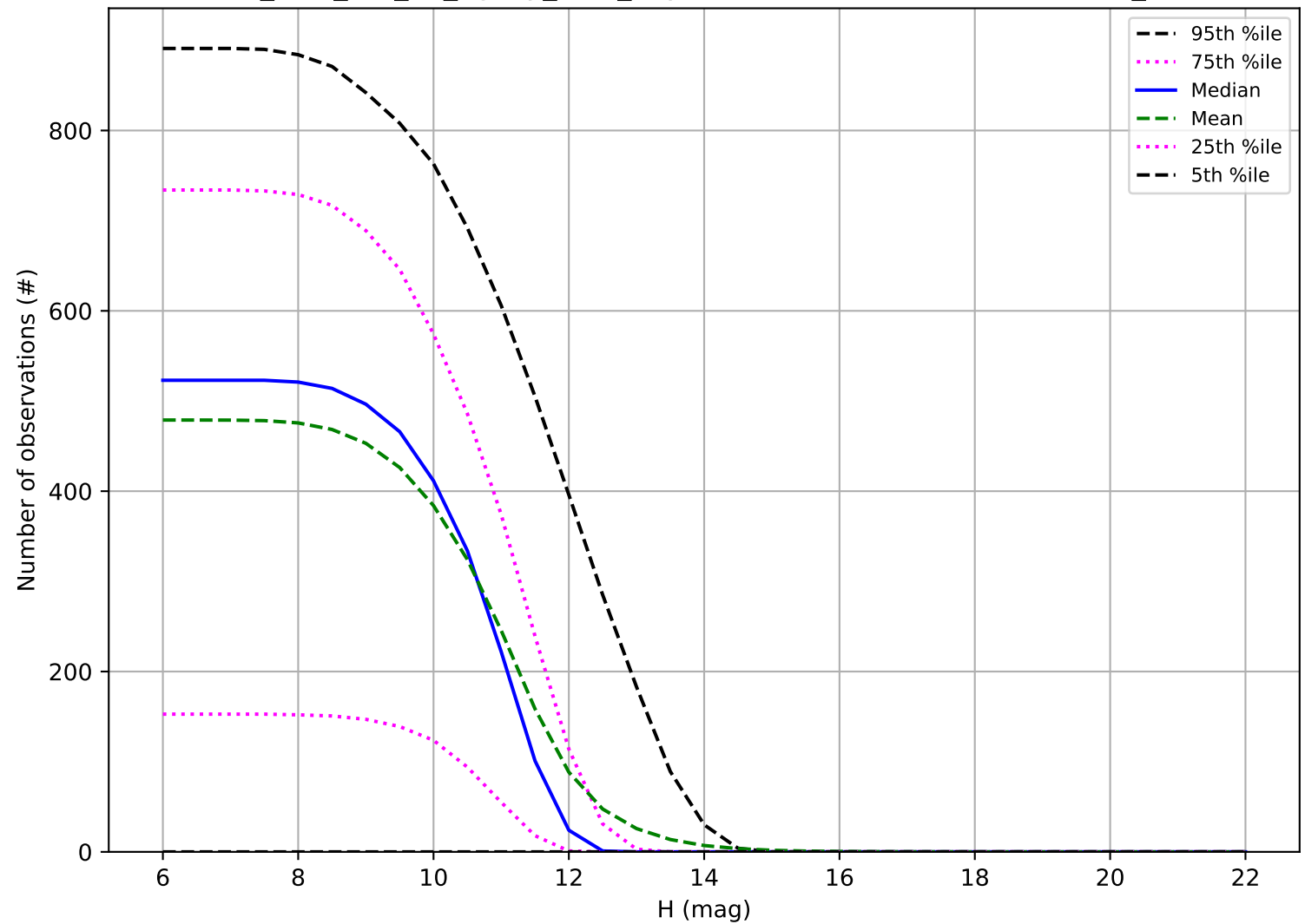
too_elab_r16_d2_ugrizy_v3.4_10yrs: Number of observations OCC_r20
