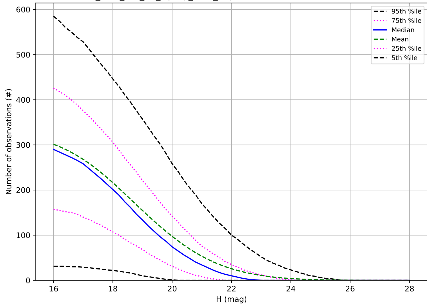
too_elab_r16_d2_ugrizy_v3.4_10yrs: Number of observations NEO
