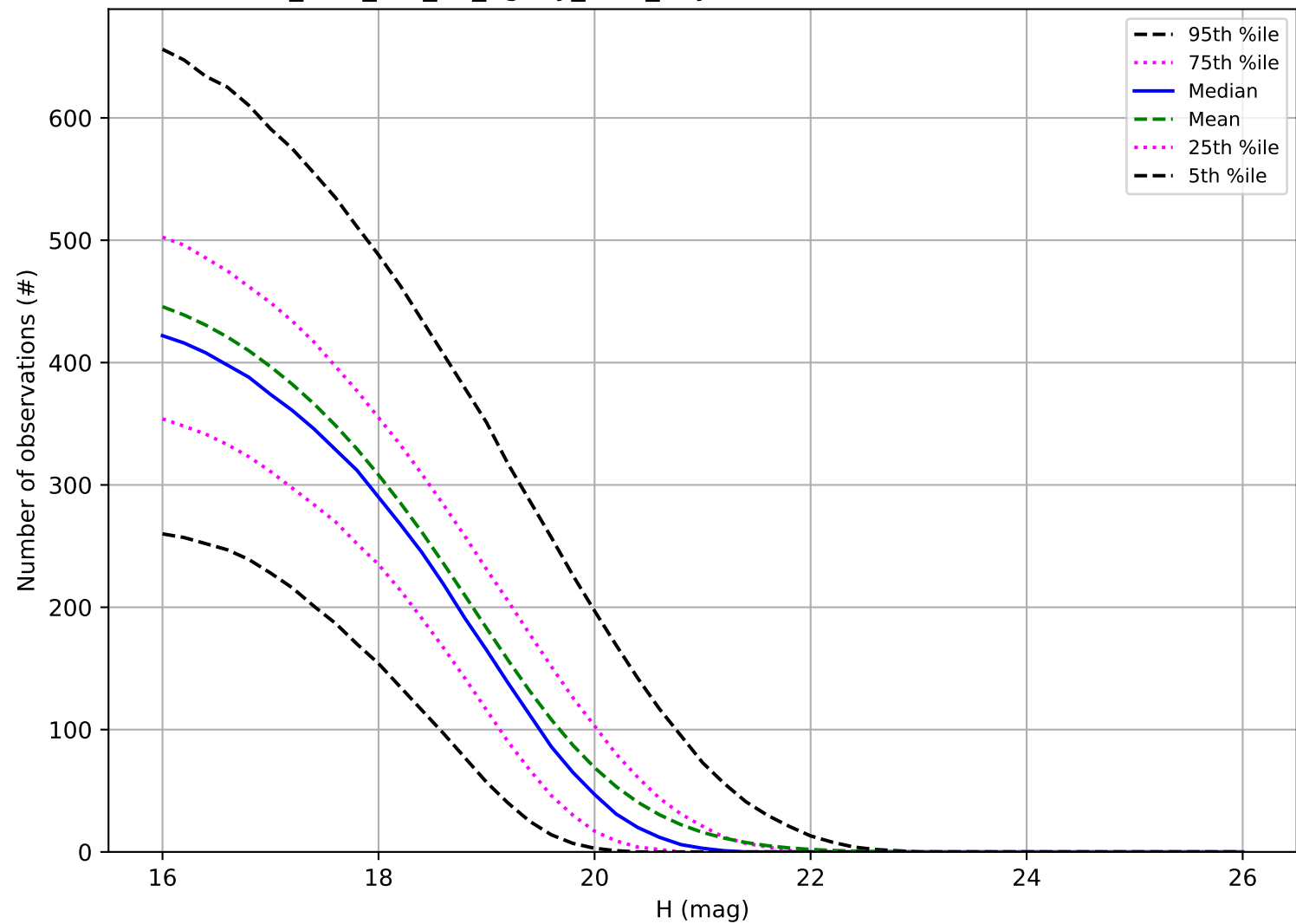
too_elab_r16_d2_ugrizy_v3.4_10yrs: Number of observations MBA
