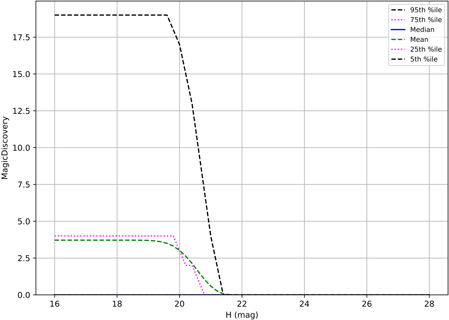
too_elab_r16_d2_ugrizy_v3.4_10yrs: Vatira 6 detections in 60 nights detection loss
