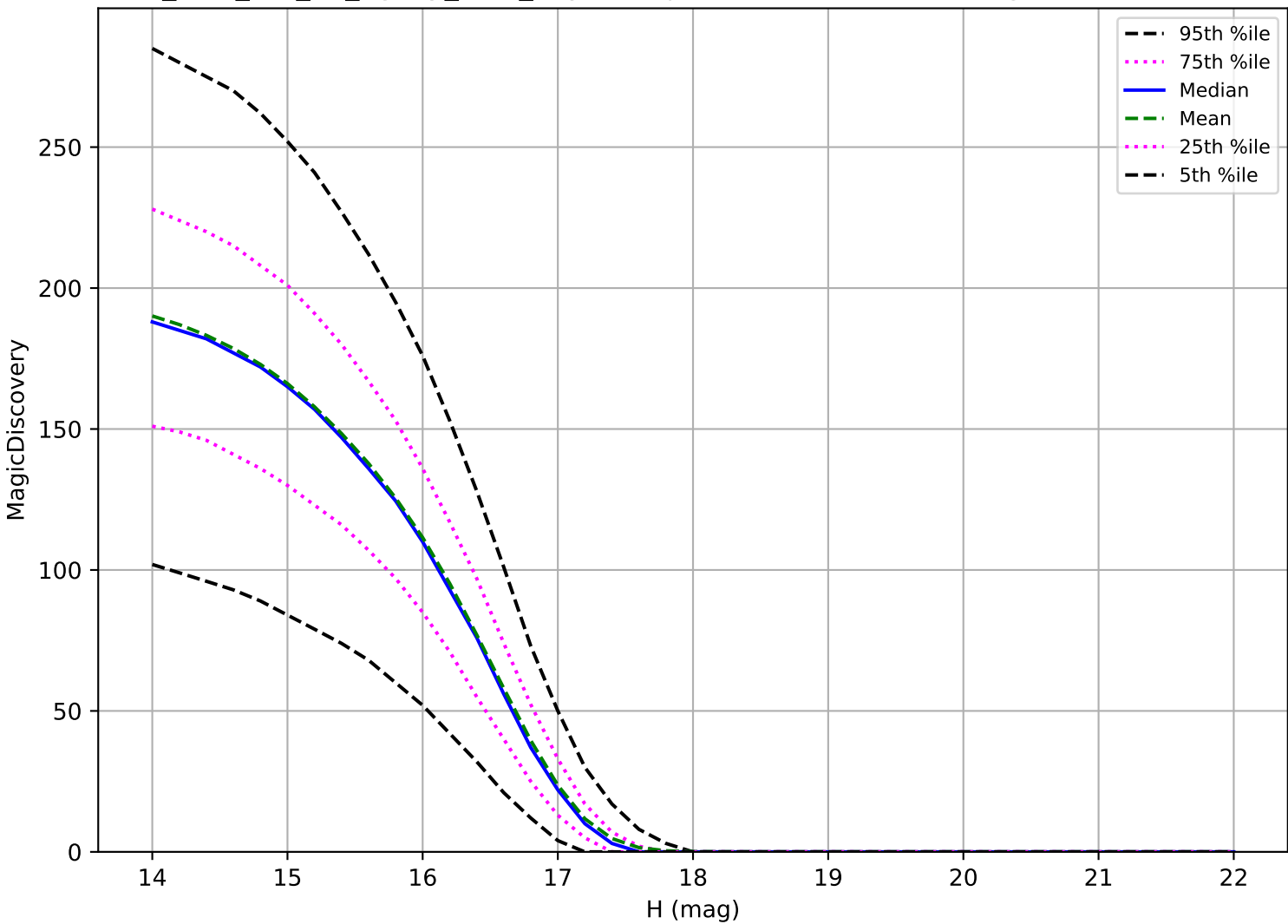
too_elab_r16_d2_ugrizy_v3.4_10yrs: Trojan 6 detections in 60 nights detection loss
