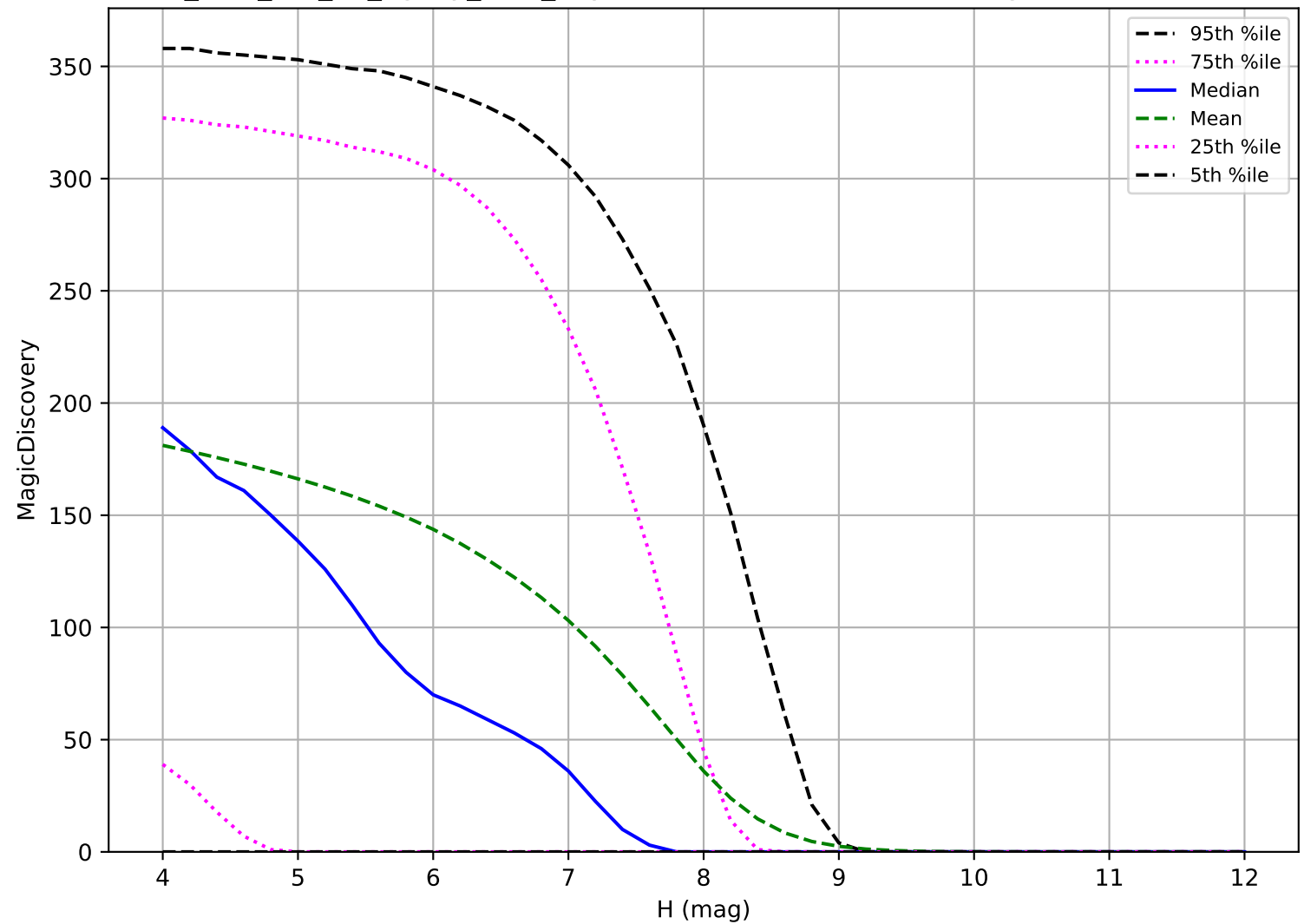
too_elab_r16_d2_ugrizy_v3.4_10yrs: TNO 6 detections in 60 nights detection loss
