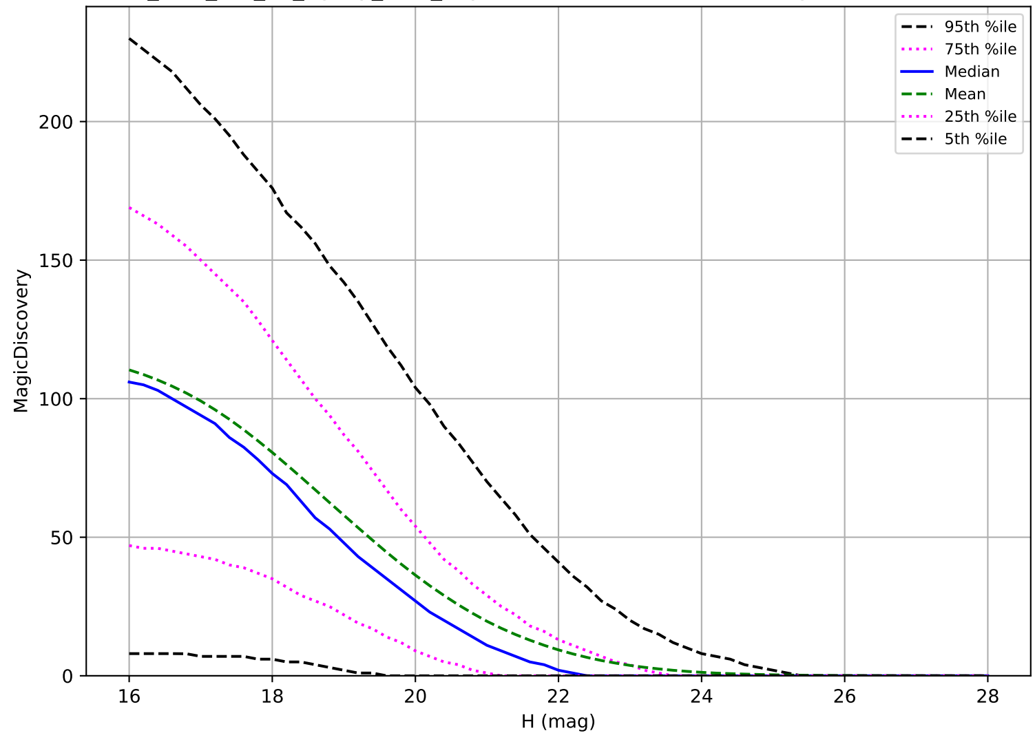
too_elab_r16_d2_ugrizy_v3.4_10yrs: PHA 6 detections in 60 nights detection loss
