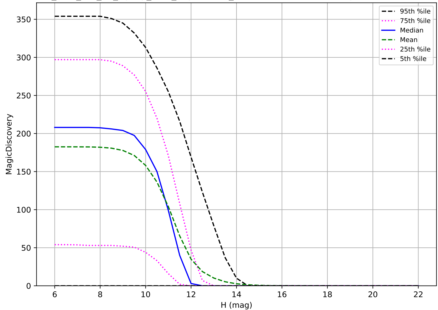
too_elab_r16_d2_ugrizy_v3.4_10yrs: OCC_r20 6 detections in 60 nights detection loss
