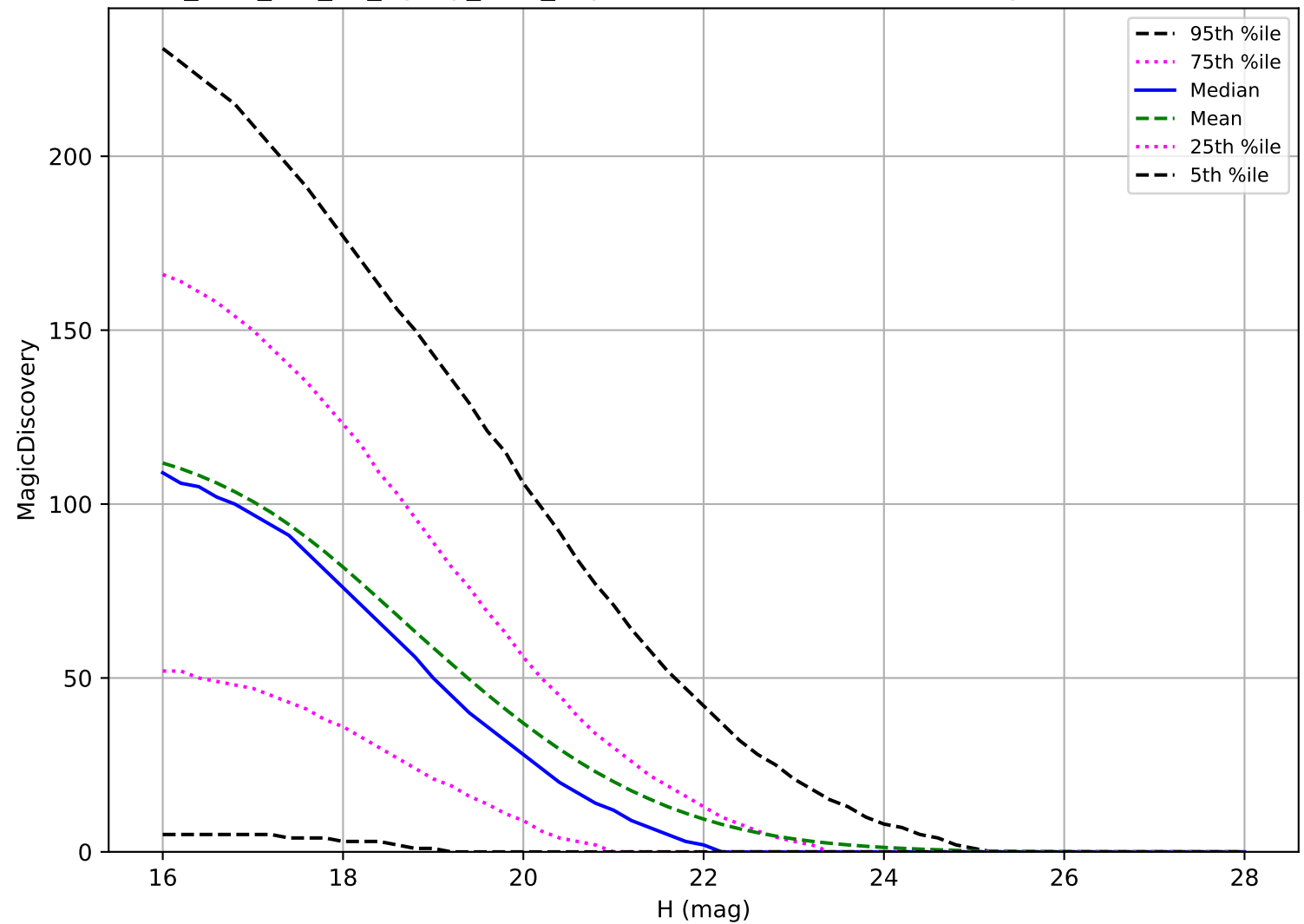
too_elab_r16_d2_ugrizy_v3.4_10yrs: NEO 6 detections in 60 nights detection loss
