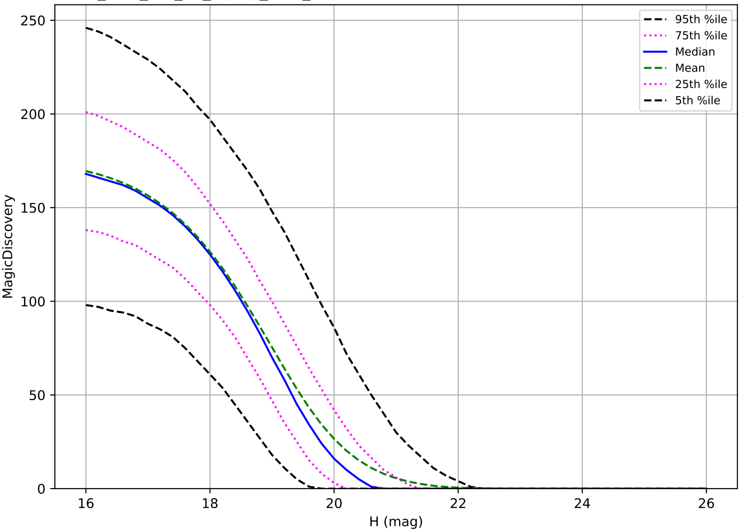
too_elab_r16_d2_ugrizy_v3.4_10yrs: MBA 6 detections in 60 nights detection loss
