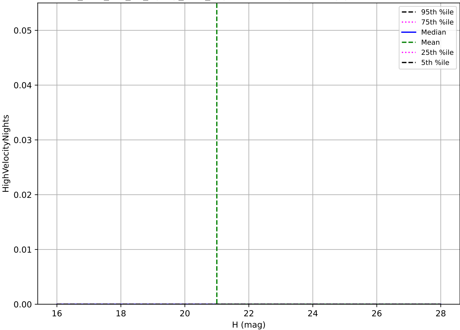
too_elab_r16_d2_ugrizy_v3.4_10yrs: Vatira High velocity pair detection loss
