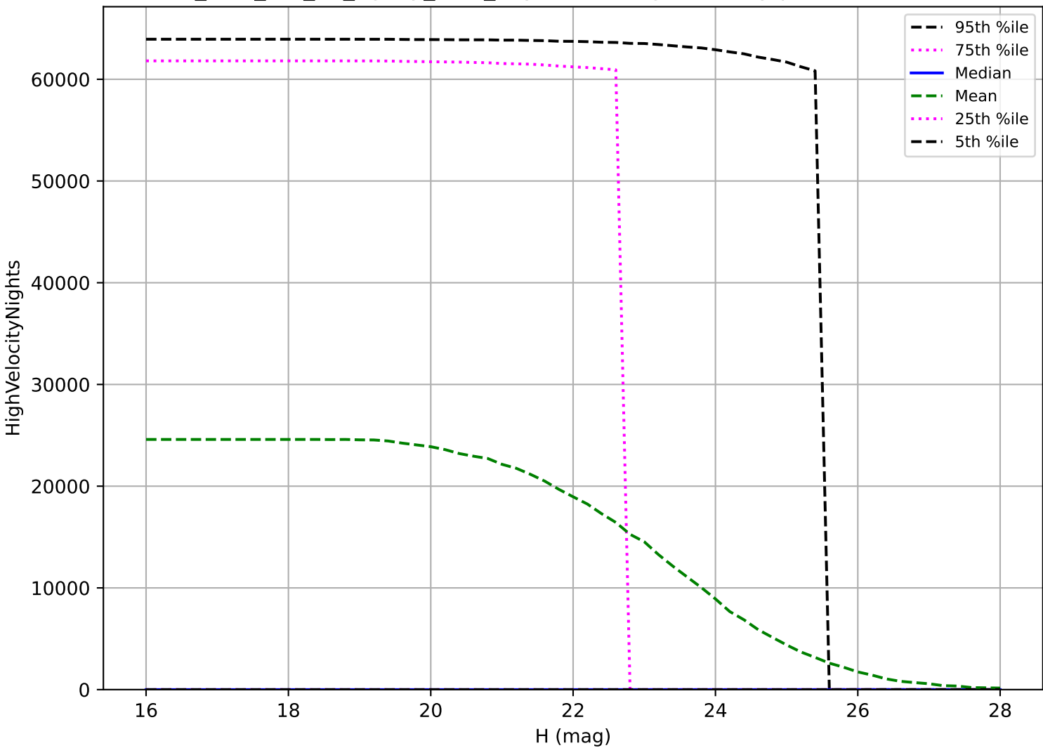
too_elab_r16_d2_ugrizy_v3.4_10yrs: PHA High velocity pair detection loss
