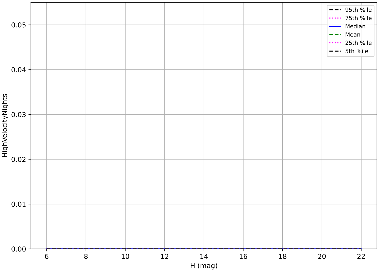
too_elab_r16_d2_ugrizy_v3.4_10yrs: OCC_r5 High velocity pair detection loss
