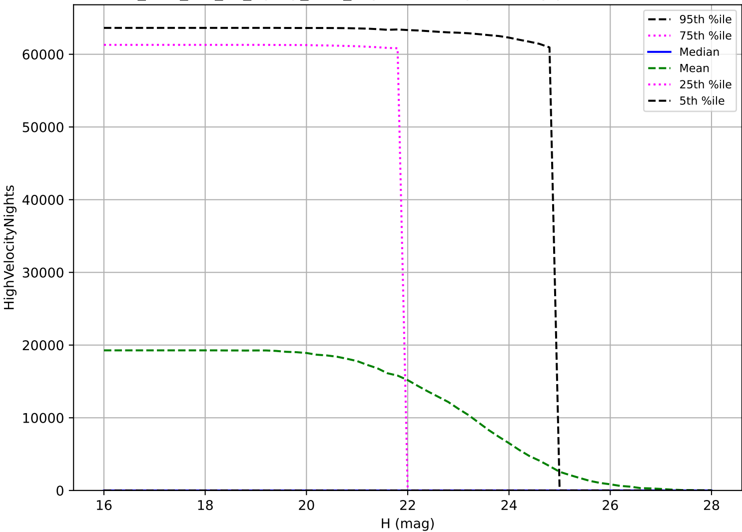
too_elab_r16_d2_ugrizy_v3.4_10yrs: NEO High velocity pair detection loss
