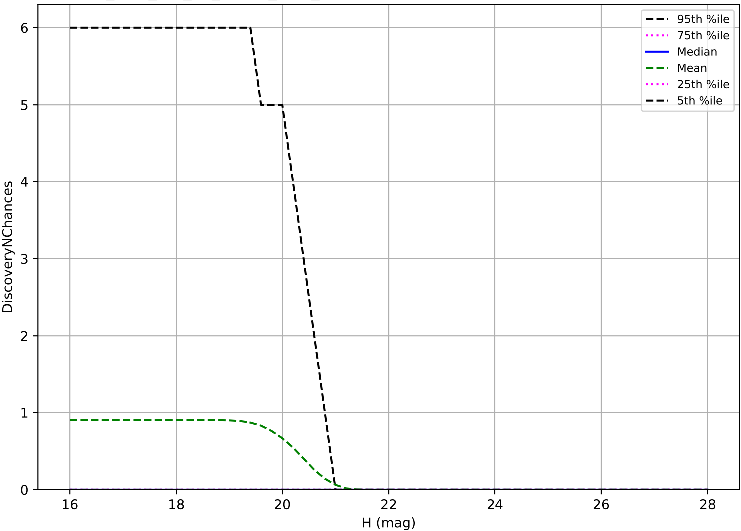
too_elab_r16_d2_ugrizy_v3.4_10yrs: Vatira 3 pairs in 15 nights detection loss
