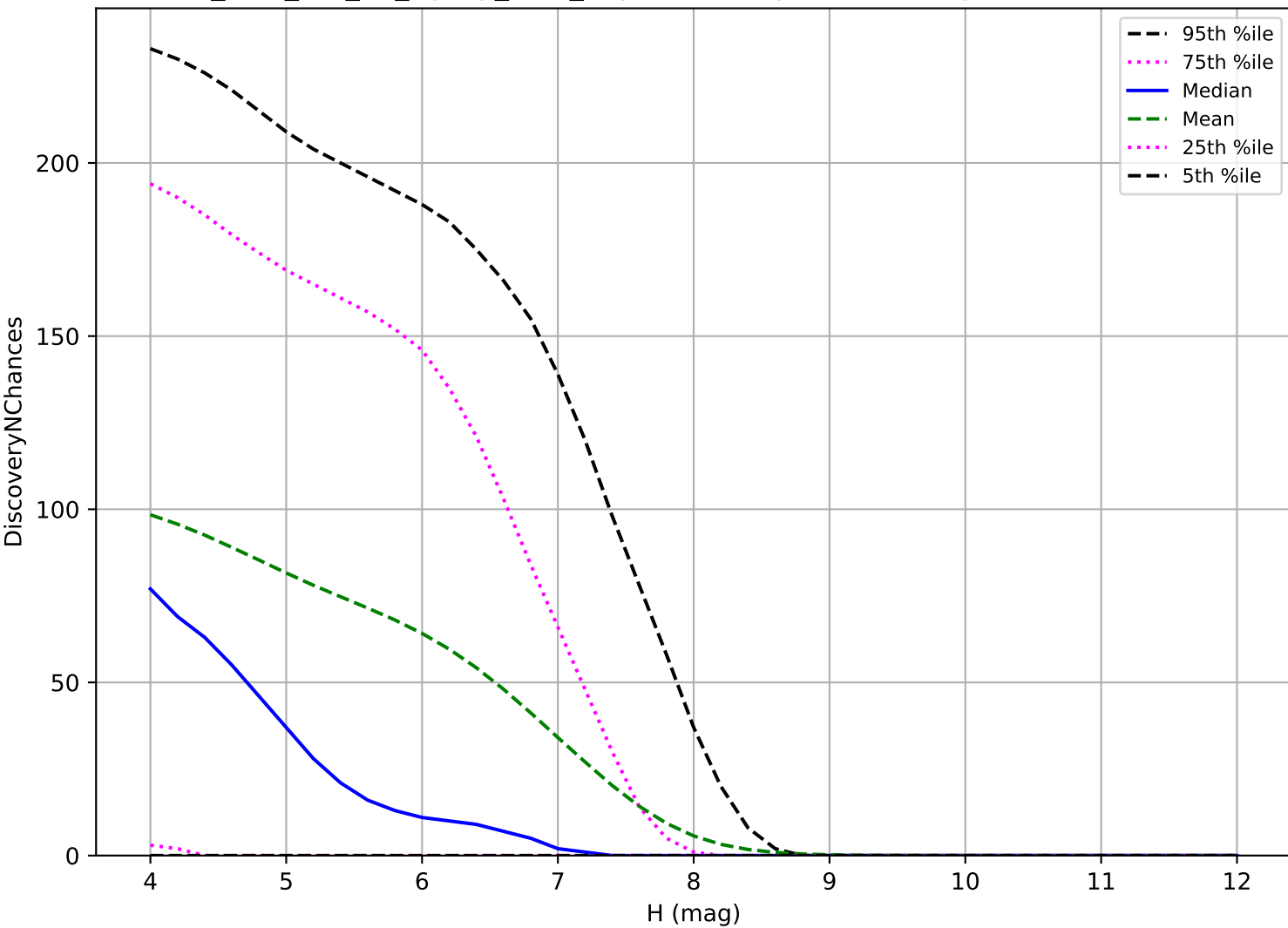
too_elab_r16_d2_ugrizy_v3.4_10yrs: TNO 3 pairs in 15 nights detection loss
