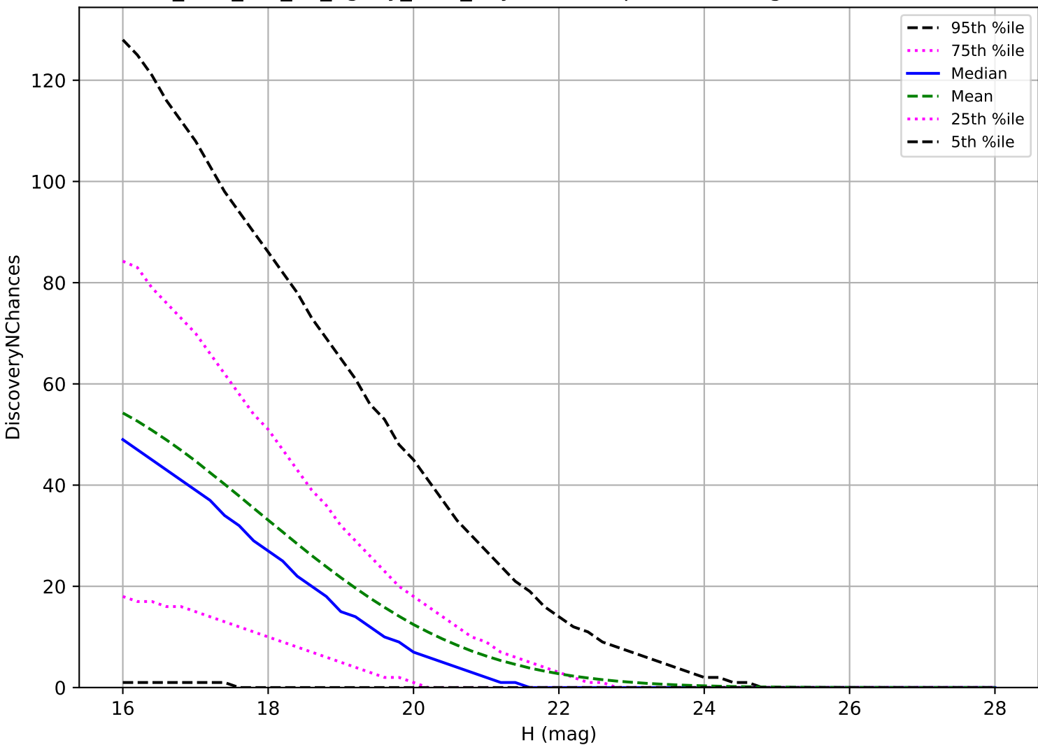
too_elab_r16_d2_ugrizy_v3.4_10yrs: PHA 3 pairs in 15 nights detection loss
