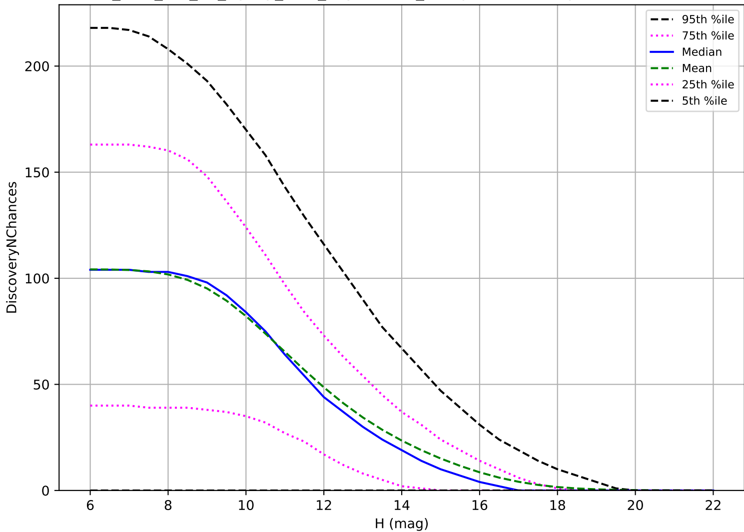
too_elab_r16_d2_ugrizy_v3.4_10yrs: OCC_r5 3 pairs in 15 nights detection loss
