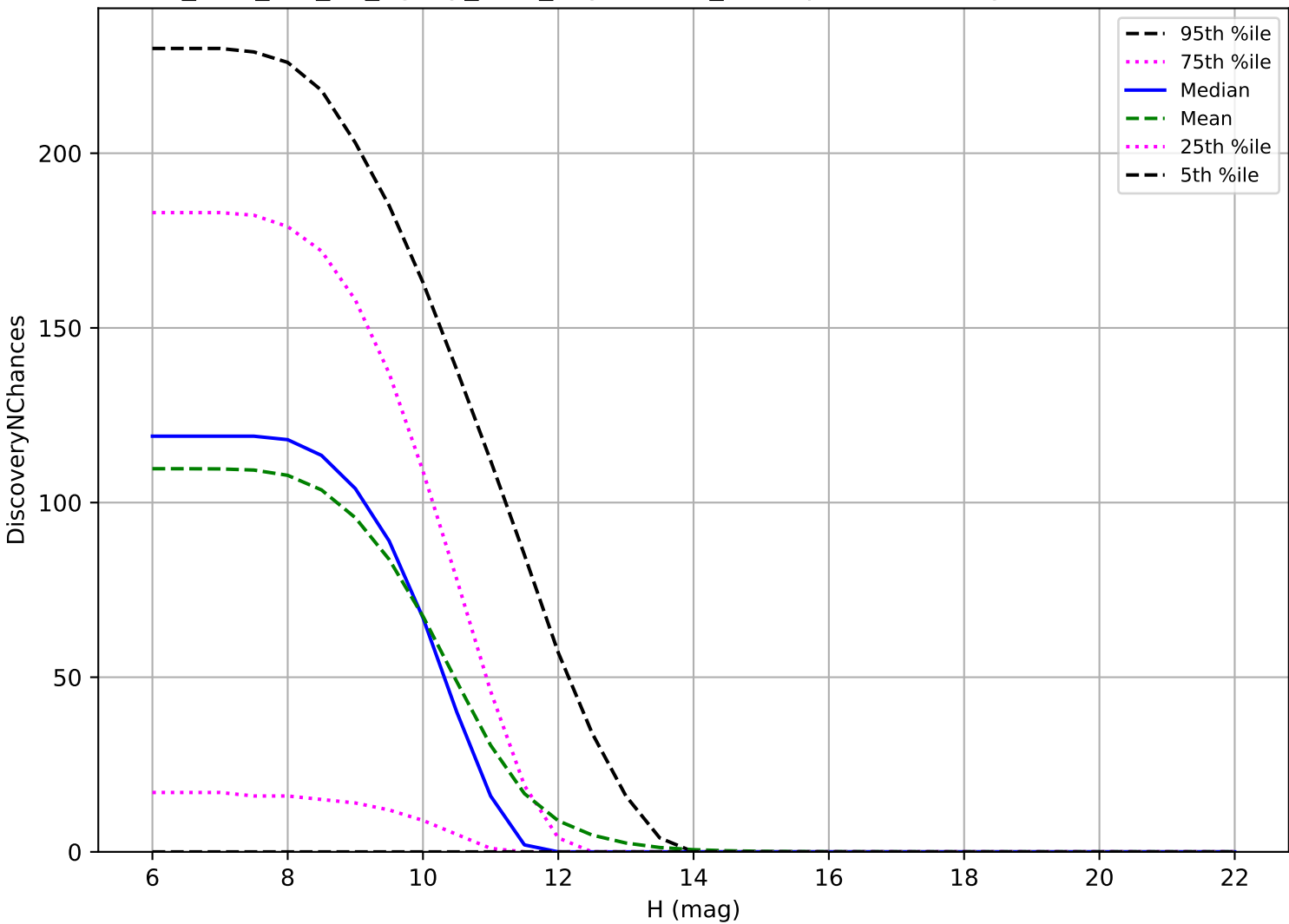
too_elab_r16_d2_ugrizy_v3.4_10yrs: OCC_r20 3 pairs in 15 nights detection loss
