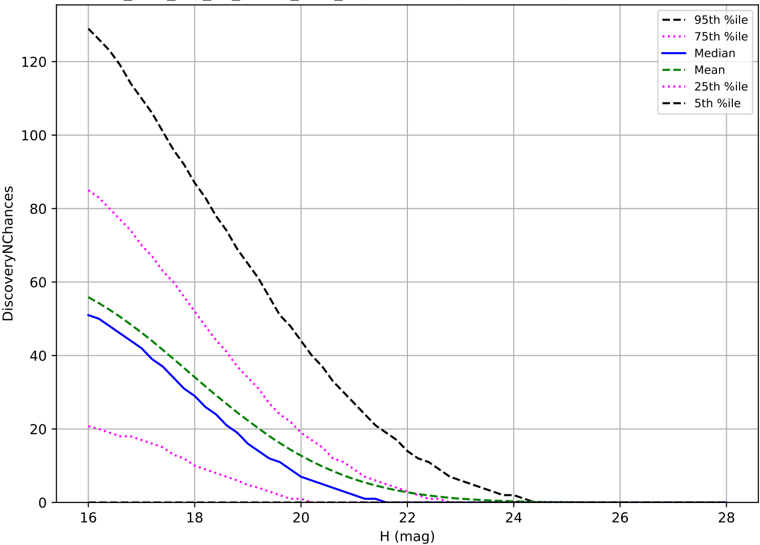
too_elab_r16_d2_ugrizy_v3.4_10yrs: NEO 3 pairs in 15 nights detection loss
