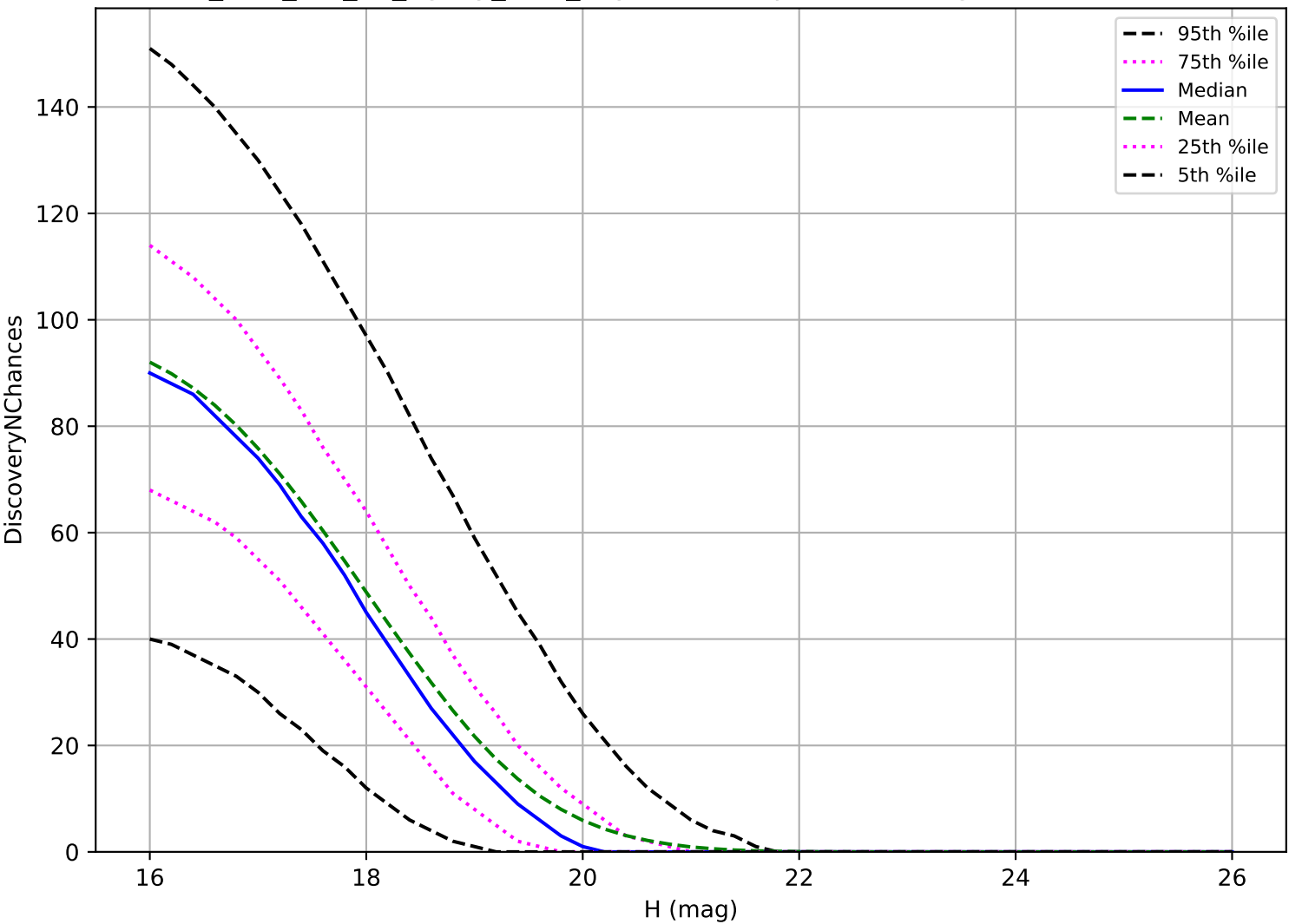
too_elab_r16_d2_ugrizy_v3.4_10yrs: MBA 3 pairs in 15 nights detection loss
