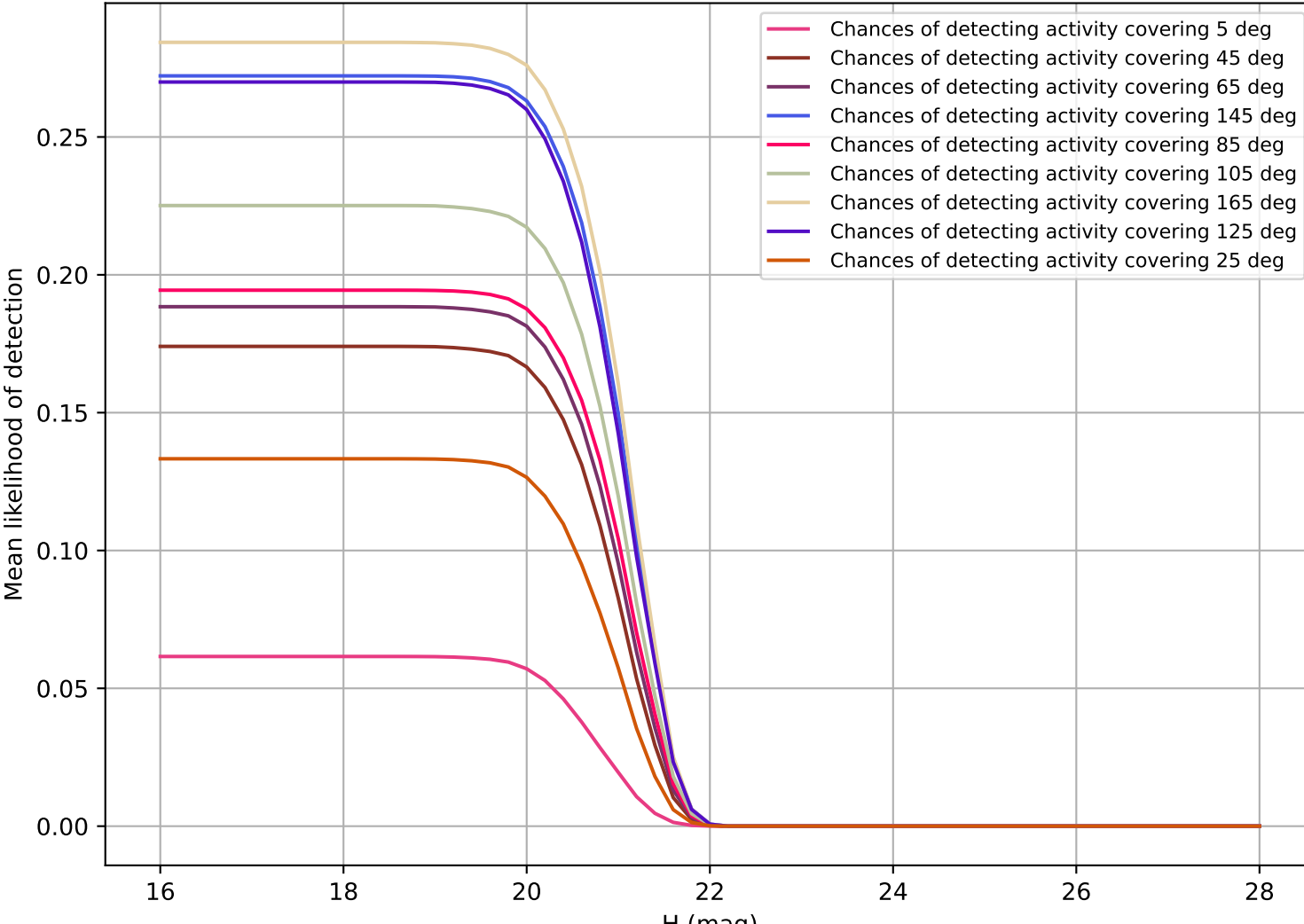
too elab r16 d2 ugrizy v3.4 10yrs Vatira
