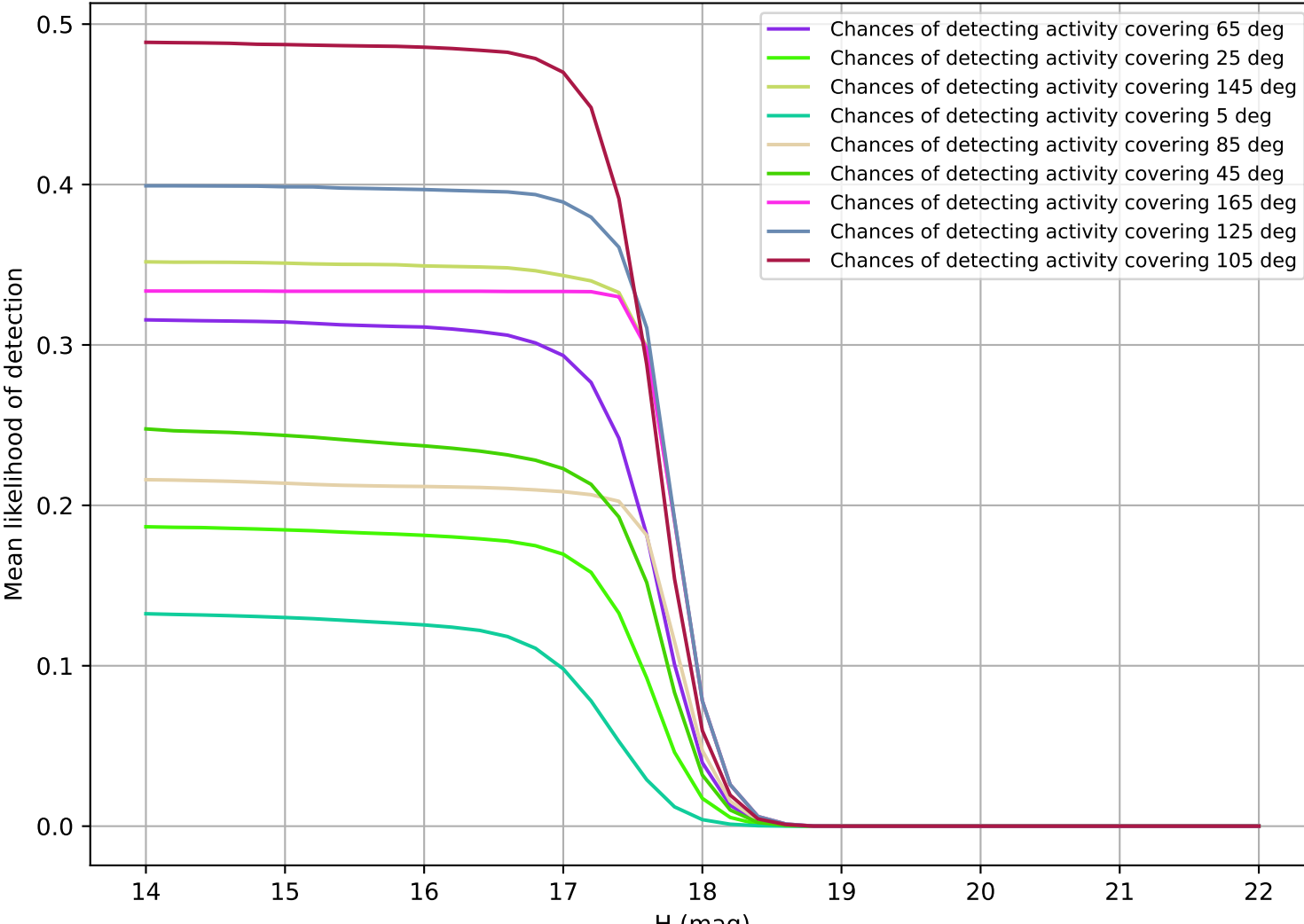
too elab r16 d2 ugrizy v3.4 10yrs Trojan
