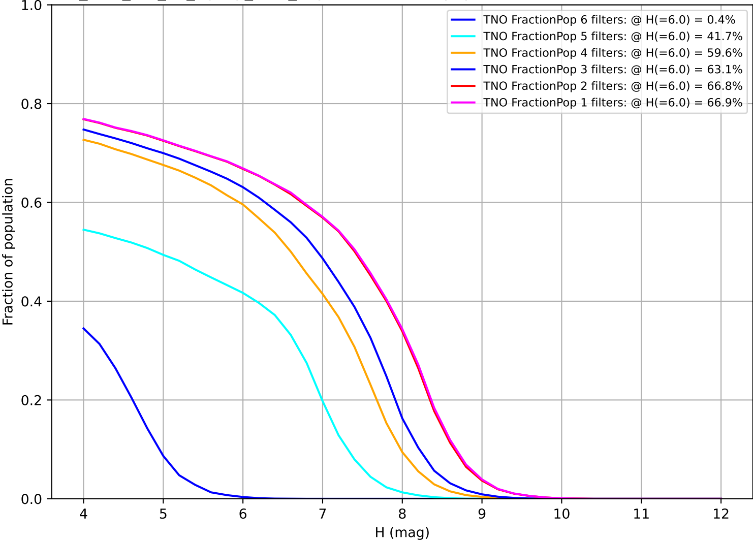
too_elab_r16_d2_ugrizy_v3.4_10yrs: Fraction of population with colors in X filters TNO
