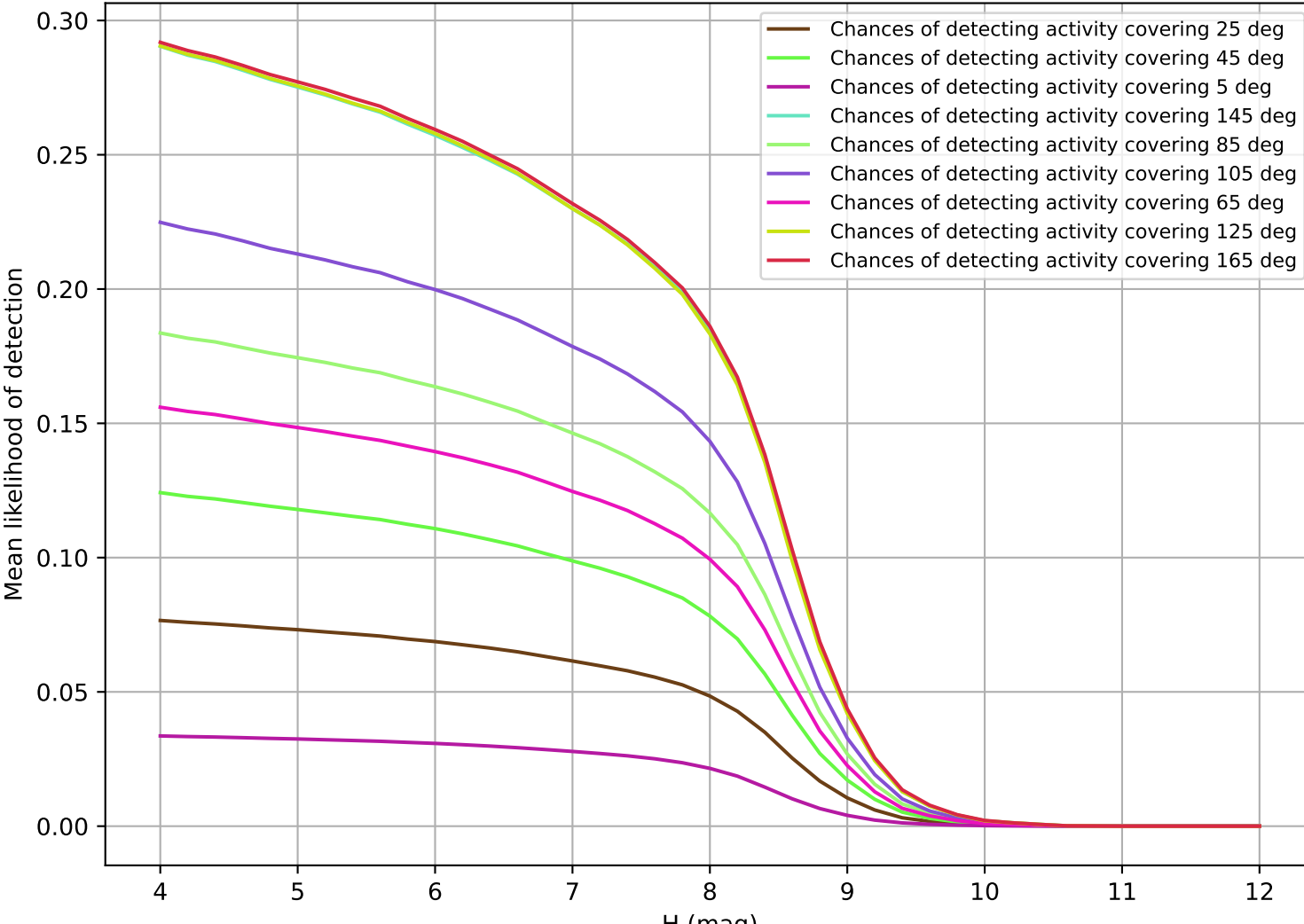
too_elab_r16_d2_ugrizy_v3.4_10yrs TNO
